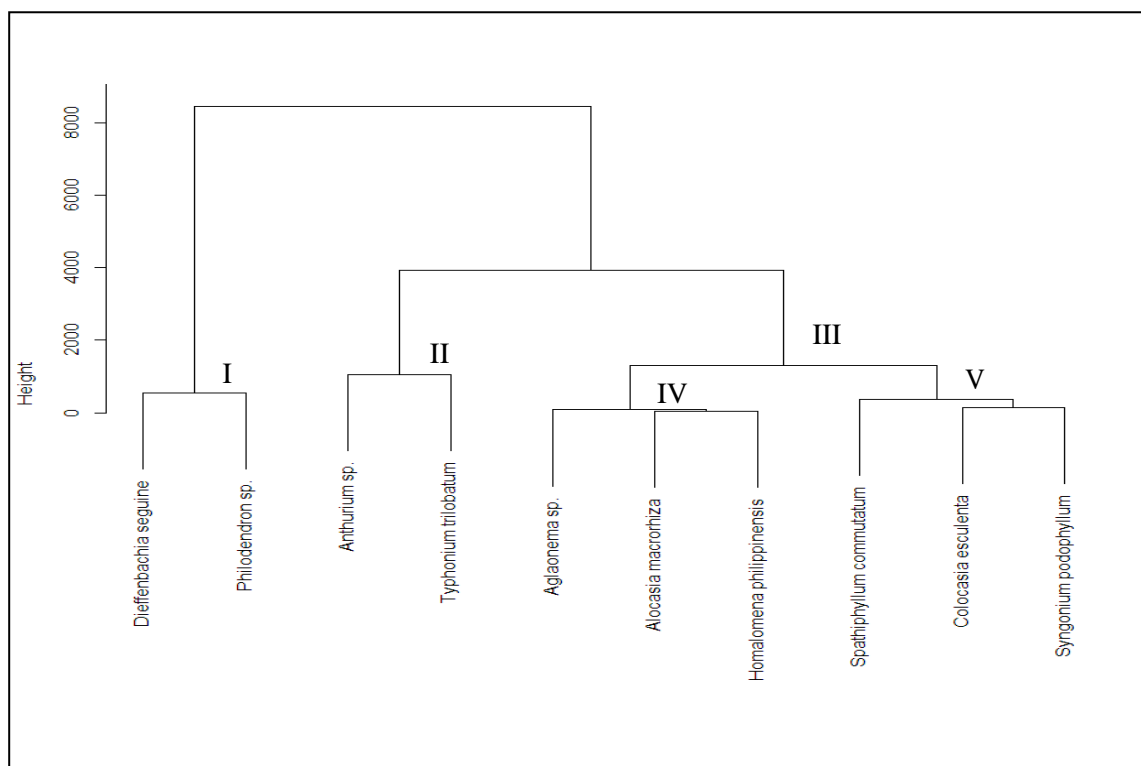
Figure 6. Dendrogram showing the relationship between the ten genera based on the type, density and size of CaOx crystals.
