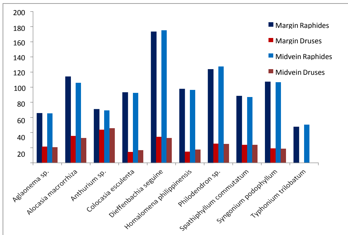
Figure 4. Comparison on the mean crystal size ( \mu\text{m} ) in different regions of the leaves of the ten genera of family Araceae.
