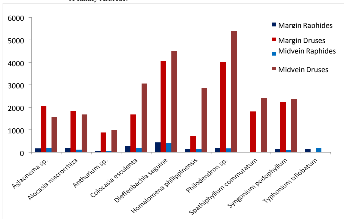
Figure 5. Comparison on the mean densities of crystals per \text{mm}^2 leaf disc in different regions of the leaves of the ten genera of family Araceae.
